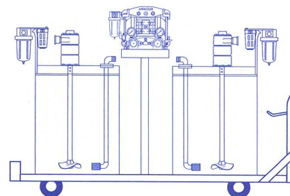
55-Gallon Dual Inlet Spray System with two 55-Gallon Cover Mixers and Cart with Bracket
