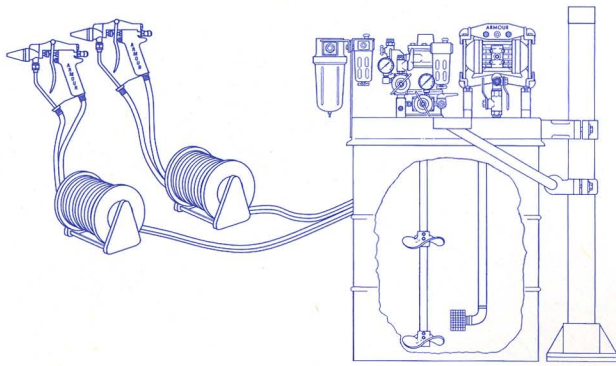
55-Gallon Dual Gun Pump Outfit with Hose Reels
