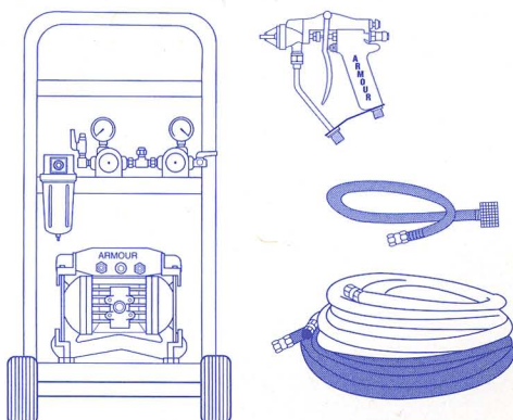
Model AR5-HVD-HT-72 Portable Pump Outfit
