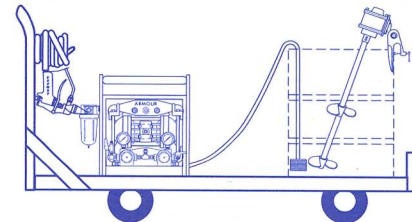
Model AR55Q Portable Pump Outfit with Model AG400 Side Mount Mixer and Model 455-C Heavy Duty Cart
